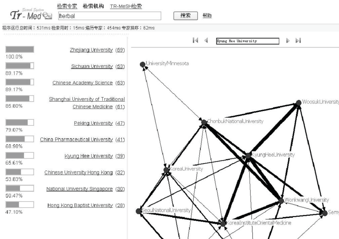
Figure 4. Retrieval interface
